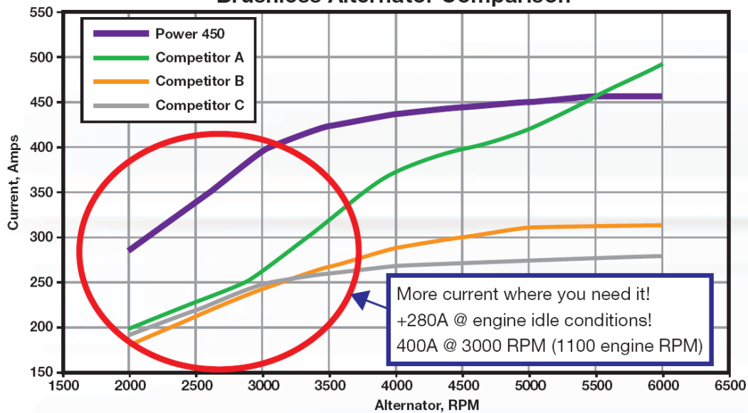
Brushless Alternator Comparison
